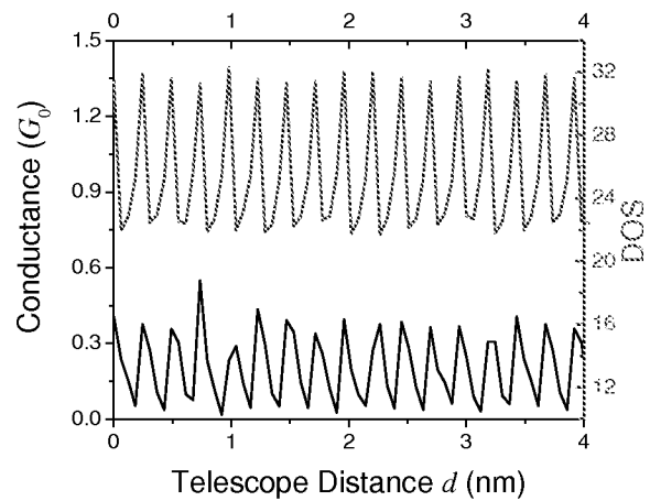
Figure 8: Periodic variations of electron conductance and density of states (DOS) with telescope distance for a (6,3)/(12,6) double-walled carbon nanotube. G_0 = 2e^2/h = 1/12.9k\Omega^{-1} .
