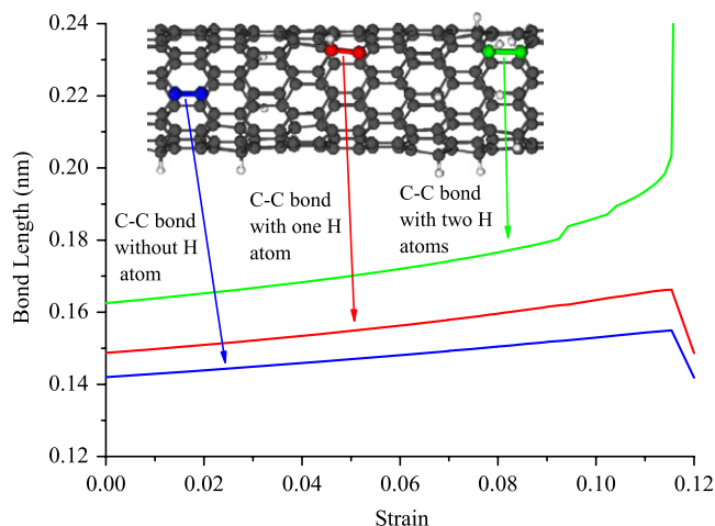
Figure 4. The bond length versus the applied strain for C–C bonds without hydrogen atom, with one H atom and with two H atoms.
