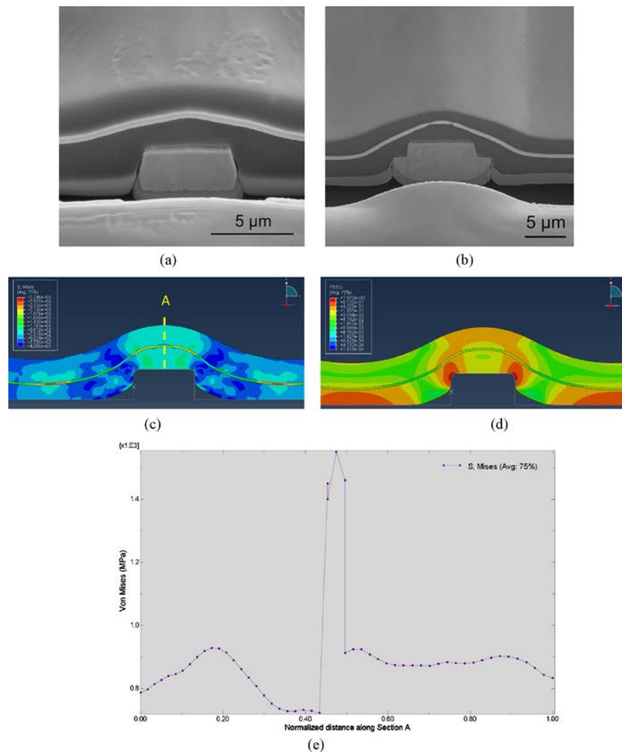
Fig. 6. The FIB/SEM images of cross sections of a laminated thin film deformed on G1000HS Mesh Grid (a) and G400HS Mesh Grid (b). The sample was tilted at 52^\circ in (a) and 40^\circ in (b). FEM results show the spatial distribution of the plastic stress (c) and strain (d) in the deformed functional structure in (a). (e) The stress discontinuity along section A in (c).
